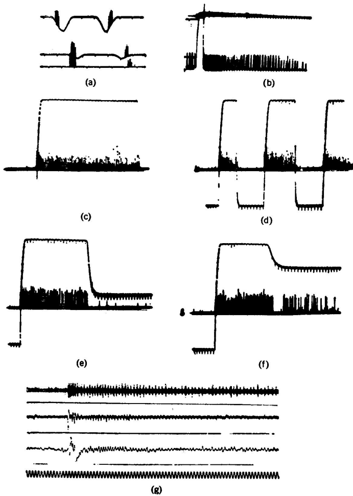
Figure 5: Operation 4) : dimming detectors. (a) This and the next frame are taken from a single fiber in the optic nerve. Here we see the response to a 7^\circ black disk passing through the receptive field. The three records are taken at three illumination levels over a 300/1 range. In the phototube record, darkening is a downward deflection. (Time marks, 5 per second.) (b) OFF and ON of light. The OFF was done shortly after one sweep began, the ON occurred a little earlier on the next sweep. The fiber is silenced completely by the ON. (Time marks, 5 per second.) (c) In this and the next three frames, we are recording from the fourth layer of endings in the
